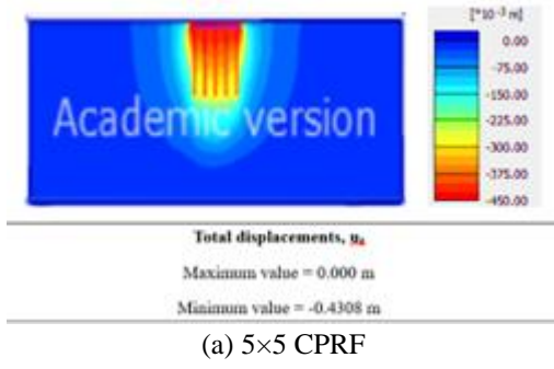
Figure A4 Vertical settlement contours using HS yield criteria
