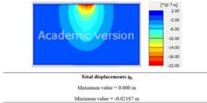
Figure A1 Contour of vertical settlement
