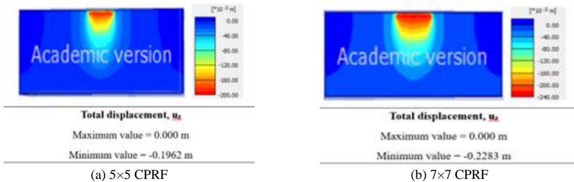
Figure A3 Contour of vertical settlement
