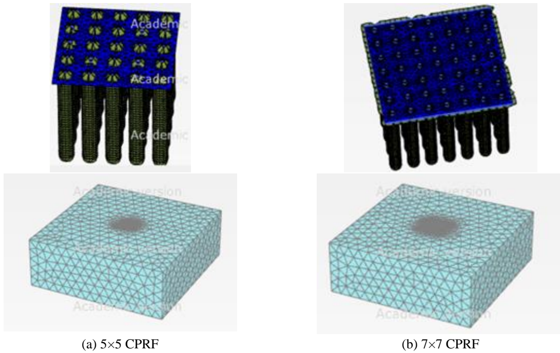
Figure A2 Schematic view and discretized mesh of CPRF
