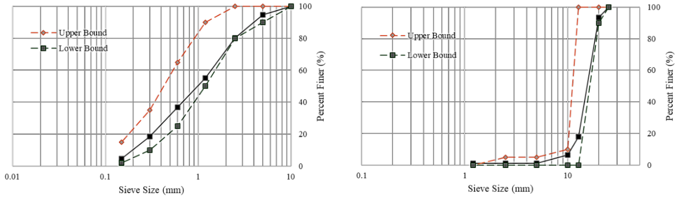
Figure 1 Gradation curve for fine and coarse aggregate
