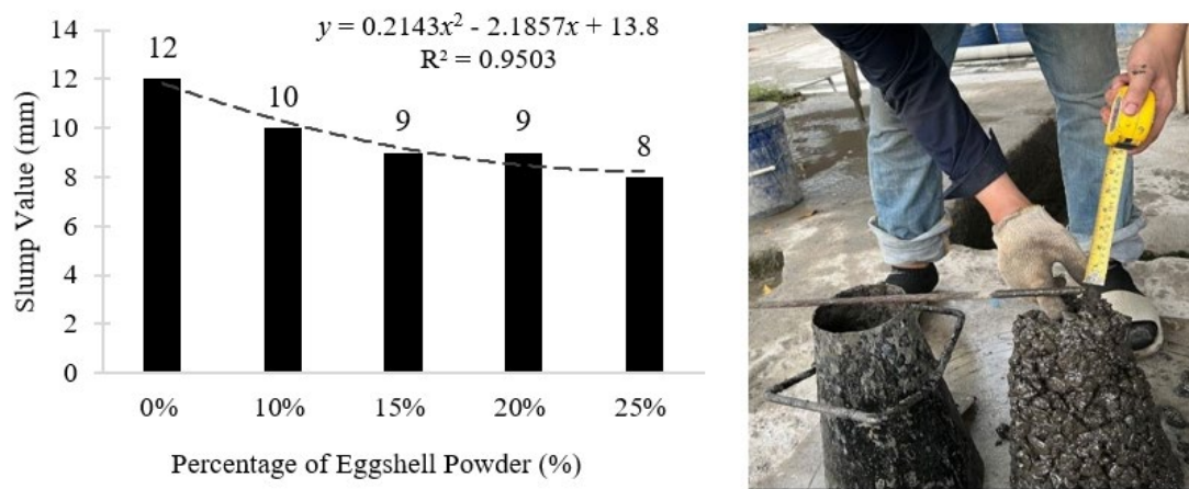
Figure 3 Slump test results
