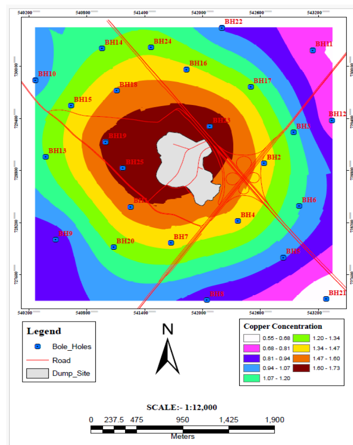
Figure 9: Spatial distribution of Copper ( \text{Cu}^{2+} ) groundwater around Olusosun Dumpsite, Lagos
