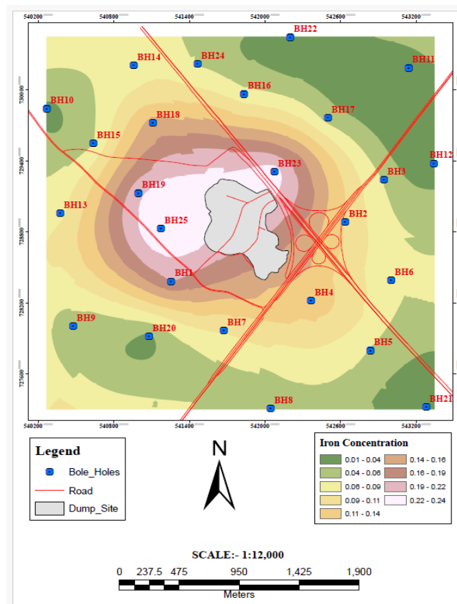
Figure 6: Spatial distribution of Iron (Fe) groundwater around Olusosun Dumpsite, Lagos
