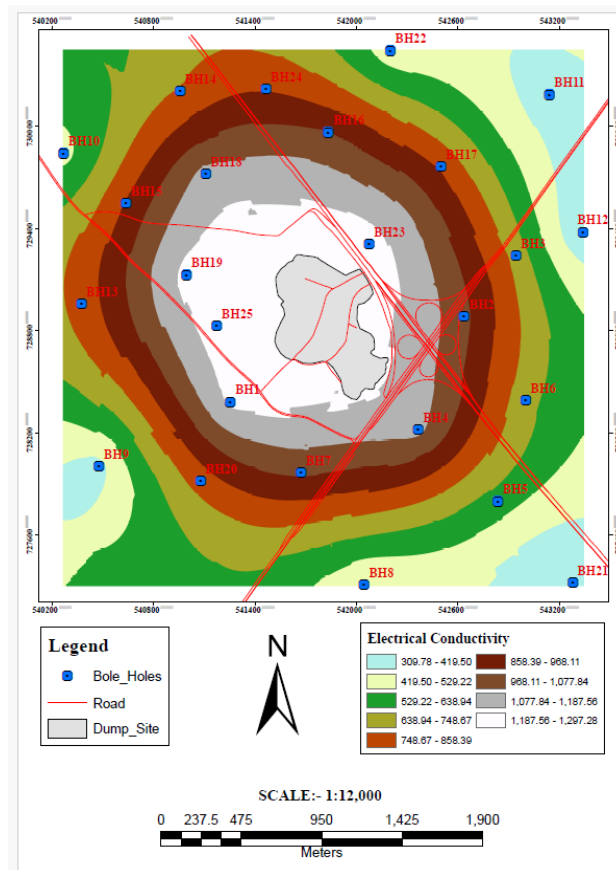
Figure 5: Spatial distribution in the EC of groundwater around Olusosun Dumpsite, Lagos
