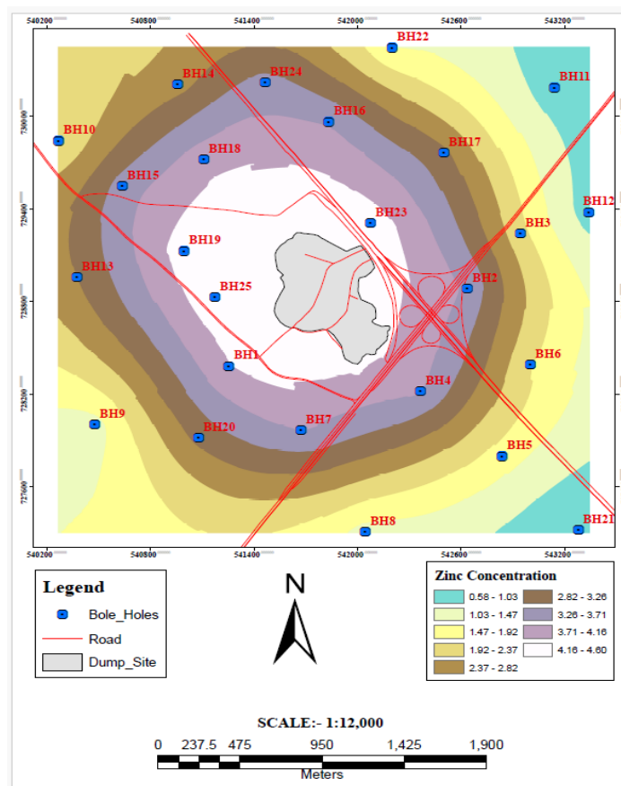
Figure 8: Spatial distribution of Zinc ( \text{Zn}^{2+} ) groundwater around Olusosun dumpsite, Lagos
