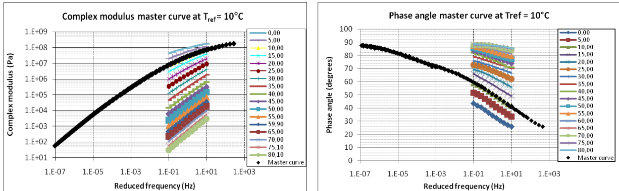
Figure 3: The |G^*| and \delta Master Curves
