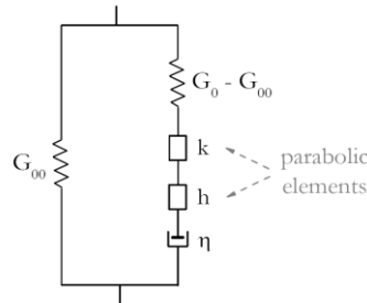
Figure 1: The 2S2P1D Model [5]
