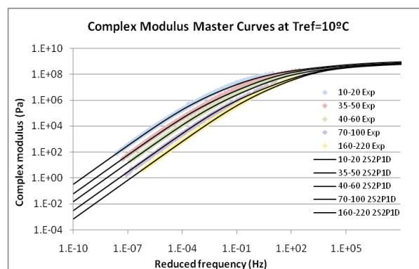
Figure 5: |G^*| Master Curves for All Samples
